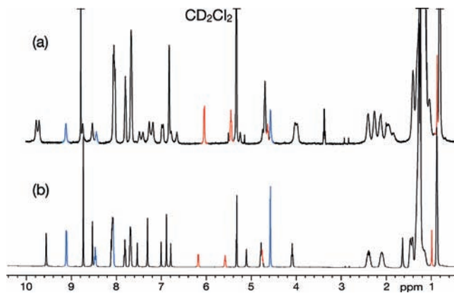
Figure 7. ^1\text{H} NMR spectra (500 MHz, \text{CD}_2\text{Cl}_2 ) of \mathbf{5a} + 3.5 equiv of PyrPic at (a) 203 and (b) 293 K (red, bound guest; blue, free guest).
