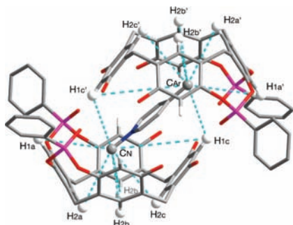
Figure 6. Main ROESY correlations observed between the bound guest and the capsular host.
