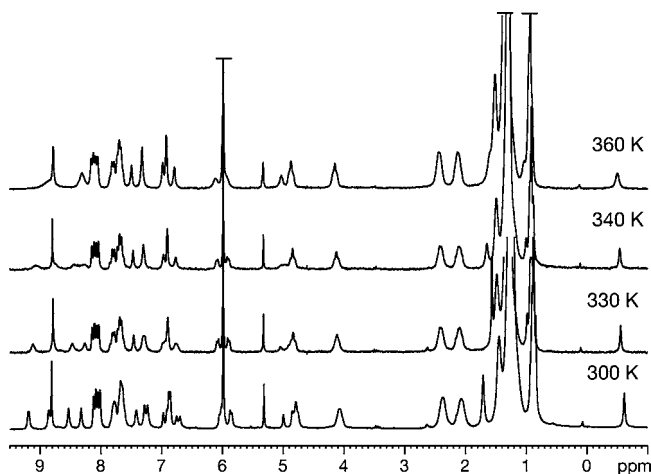
Figure 8. VT ^1\text{H} NMR spectra (200 MHz, \text{C}_2\text{D}_2\text{Cl}_4 ) of \mathbf{5a} + 0.5 equiv of PicoPic.
