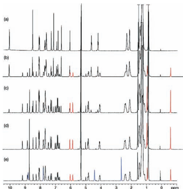
Figure 3. ^1\text{H} NMR spectra (500 MHz, \text{CD}_2\text{Cl}_2 , 293 K) of (a) free host 5a , (b) 5a + 0.2 equiv of PicoPic, (c) 5a + 0.4 equiv of PicoPic, (d) 5a + 0.5 equiv of PicoPic, and (e) 5a + 1.3 equiv of PicoPic. Colors: red, bound picolinium; blue, free picolinium.
