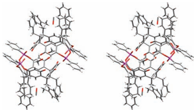
Figure 4. Stereoview of the X-ray structure of the capsular dimeric assembly [5b \cdot CH_3OH]_2 .
