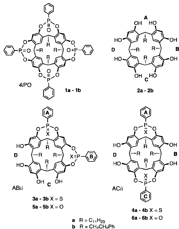
Figure 1. Structures of the 4 i PO phosphorylated cavitands 1 and the 2 i PO phosphorylated cavitands AB ii ( 3 and 5 ) and AC ii ( 4 and 6 ). The labels AB and AC indicate the proximal and distal positions of the two phosphorus groups in the 2 i derivatives.
