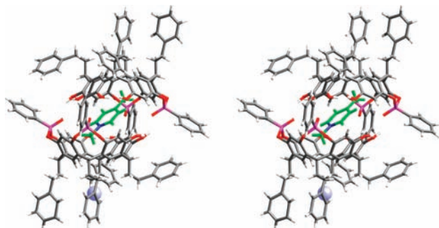
Figure 5. Stereoview of the X-ray structure of the supramolecular complex PicoIod@(5b)_2 .
