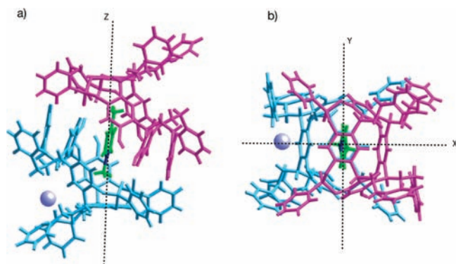
Figure 10. (a) Side and (b) top views of the X-ray structure of PicoIod@(5b) _2 that emphasize the formation of the supramolecular rotor.
