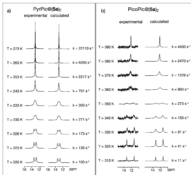
Figure 9. Experimental and calculated ^{31}\text{P} NMR spectra at different temperatures for (a) 5\mathbf{a} + 1 equiv of PyrPic in \text{CD}_2\text{Cl}_2 and (b) 5\mathbf{a} + 1 equiv of PicoPic in \text{C}_2\text{D}_2\text{Cl}_4 .
