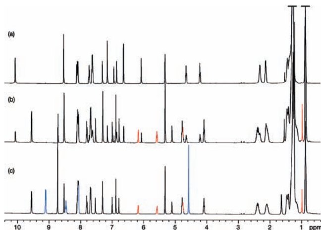
Figure 2. ^1\text{H} NMR spectra (500 MHz, \text{CD}_2\text{Cl}_2 , 293 K) of (a) free host 5a , (b) 5a + 0.3 equiv of PyrPic, and (c) 5a + 3.5 equiv of PyrPic. Colors: red, bound pyridinium; blue, free pyridinium.
